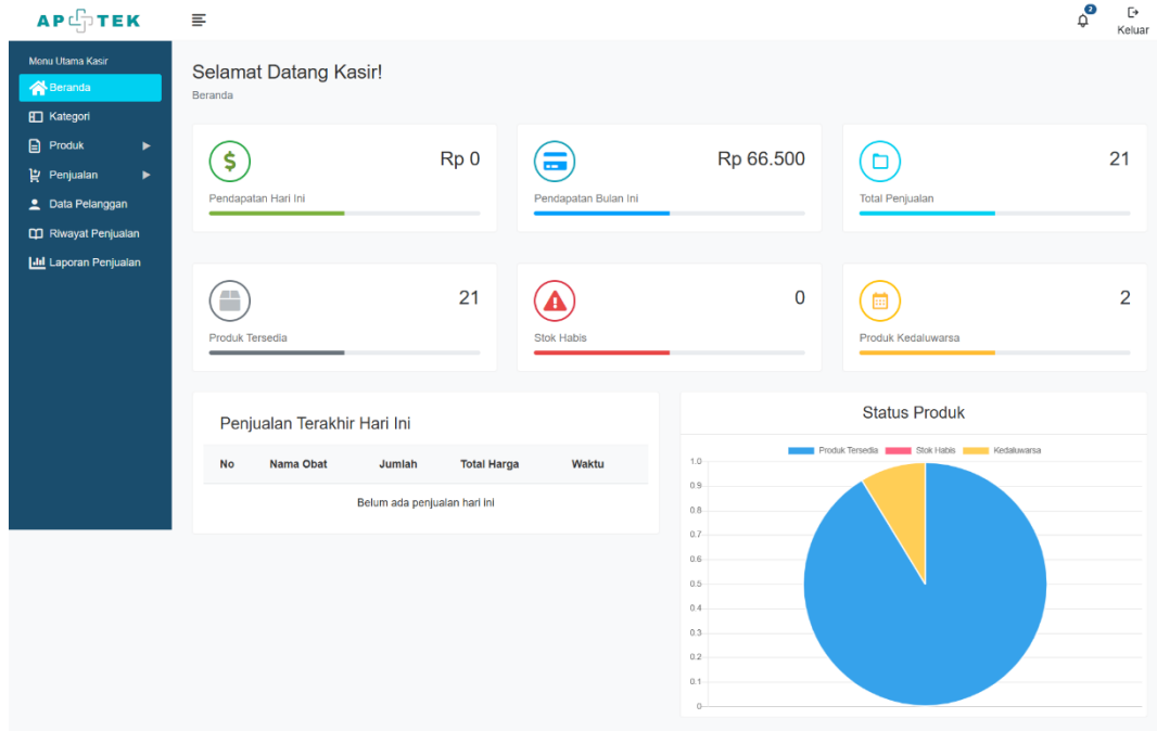
Gambar 3. Menu Samping
