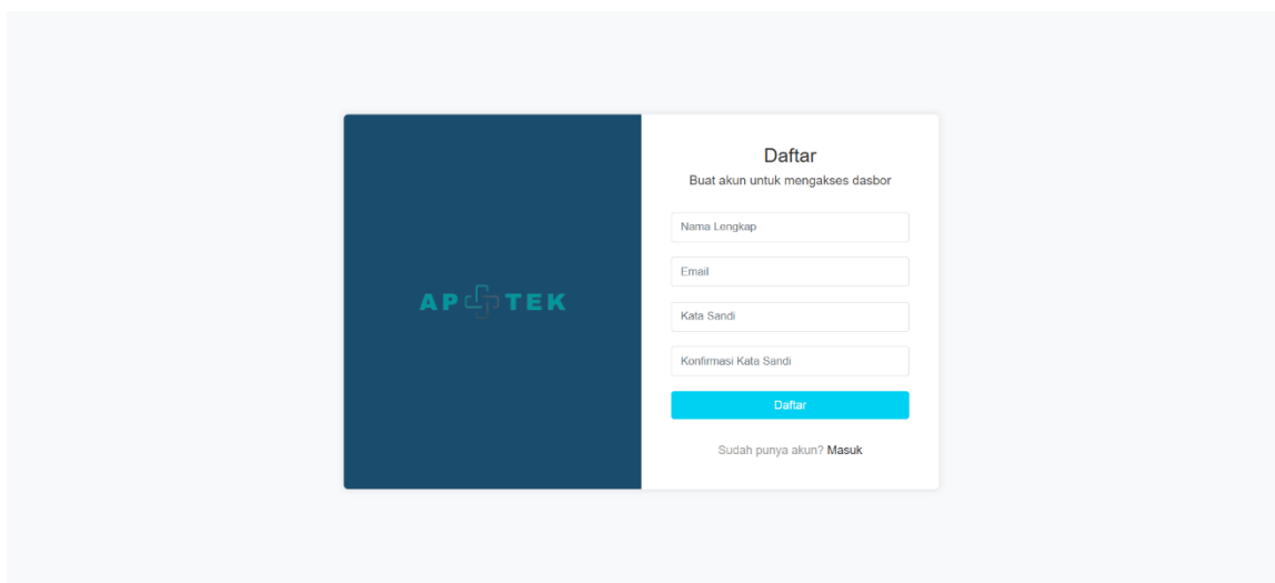
Gambar 2. Register
